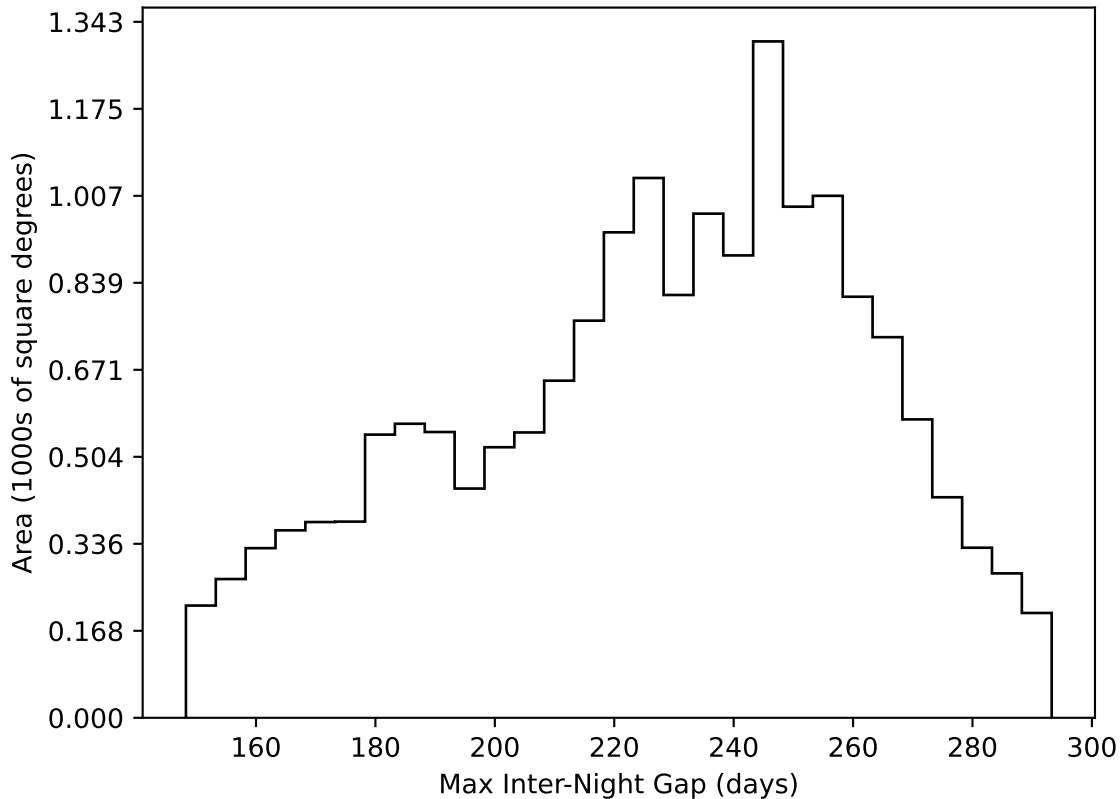
start_date_do180v3.4_10yrs WFD all bands: Max Inter-Night Gap
