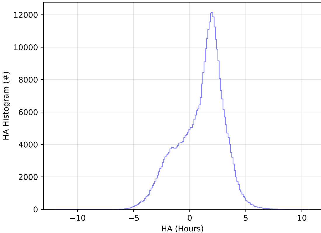
start_date_do180v3.4_10yrs WFD y band: HA Histogram
