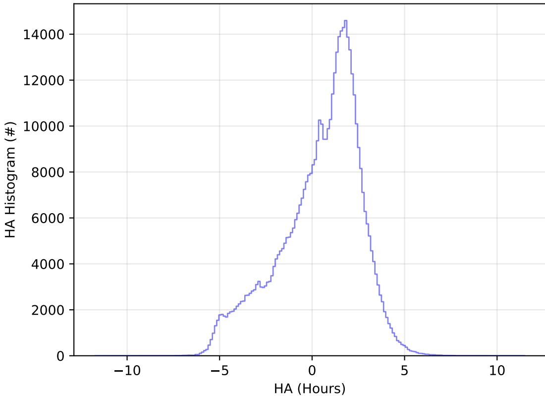
start_date_do180v3.4_10yrs All sky r band: HA Histogram
