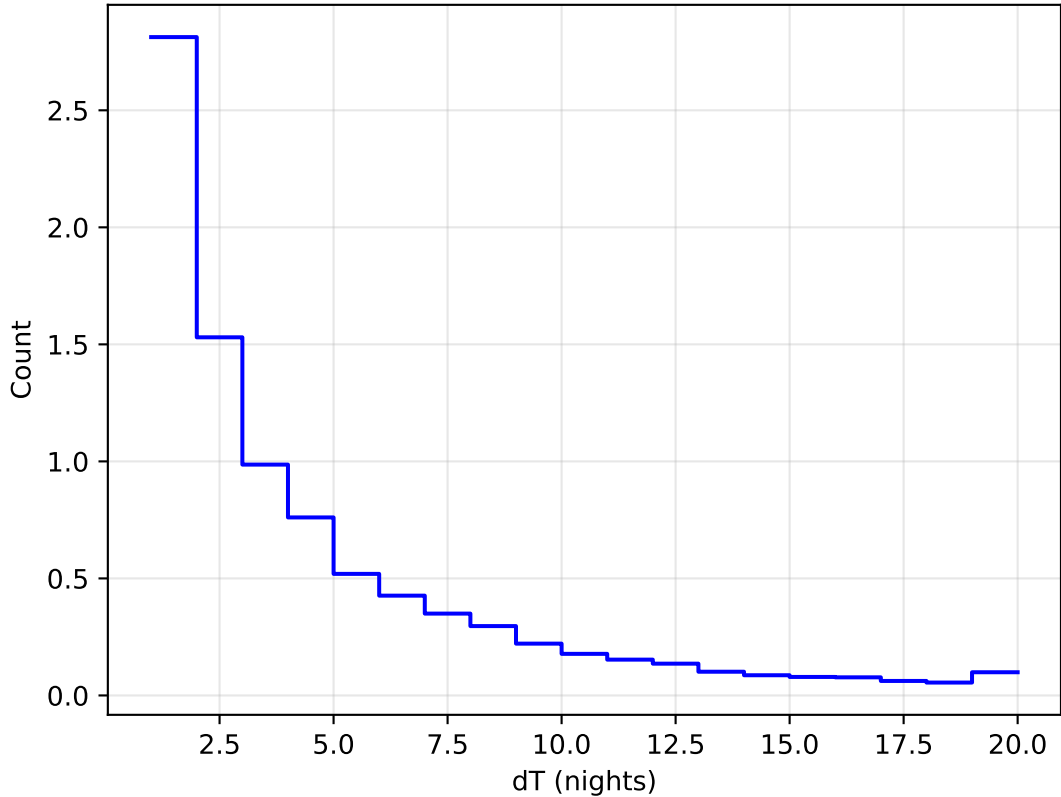
start_date_do180v3.4_10yrs All sky all bands: DeltaNight Histogram 1e6
