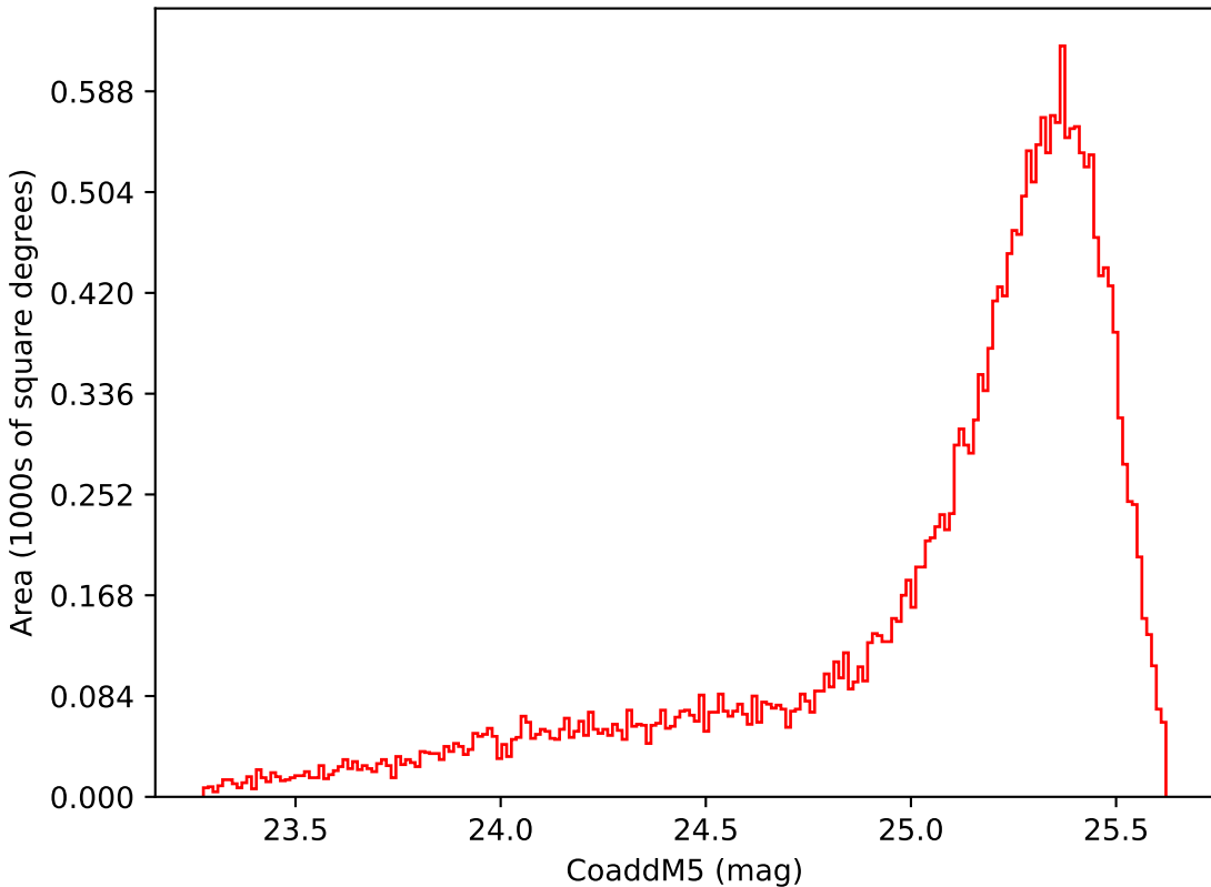
start_date_do180v3.4_10yrs Yr 1 i band: CoaddM5
