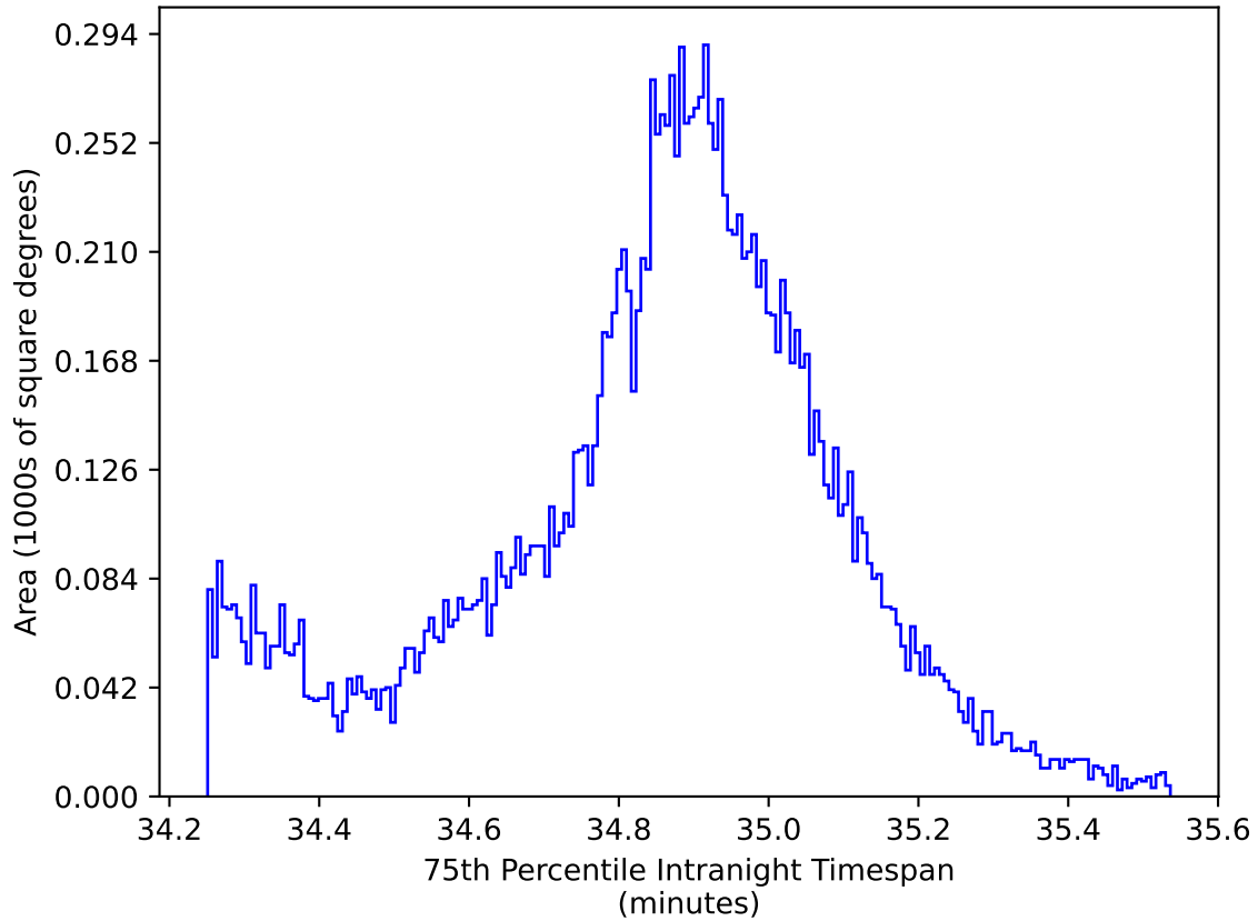
start_date_do180v3.4_10yrs WFD all bands: 75th Percentile Intranight Timespan
