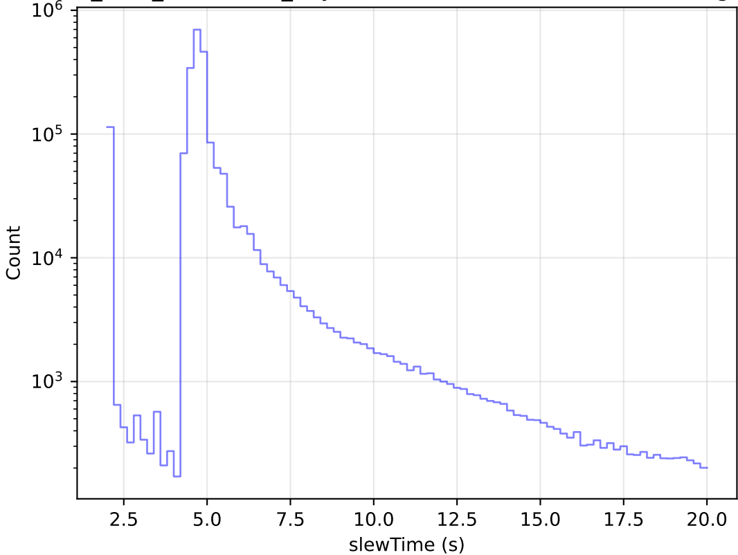
start_date_do180v3.4_10yrs All visits: Zoom Slew Time Histogram
