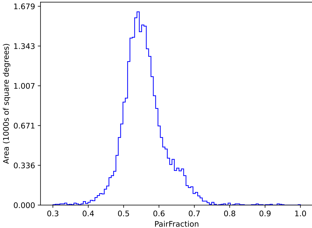
start_date_do180v3.4_10yrs (g or r or i): PairFraction
