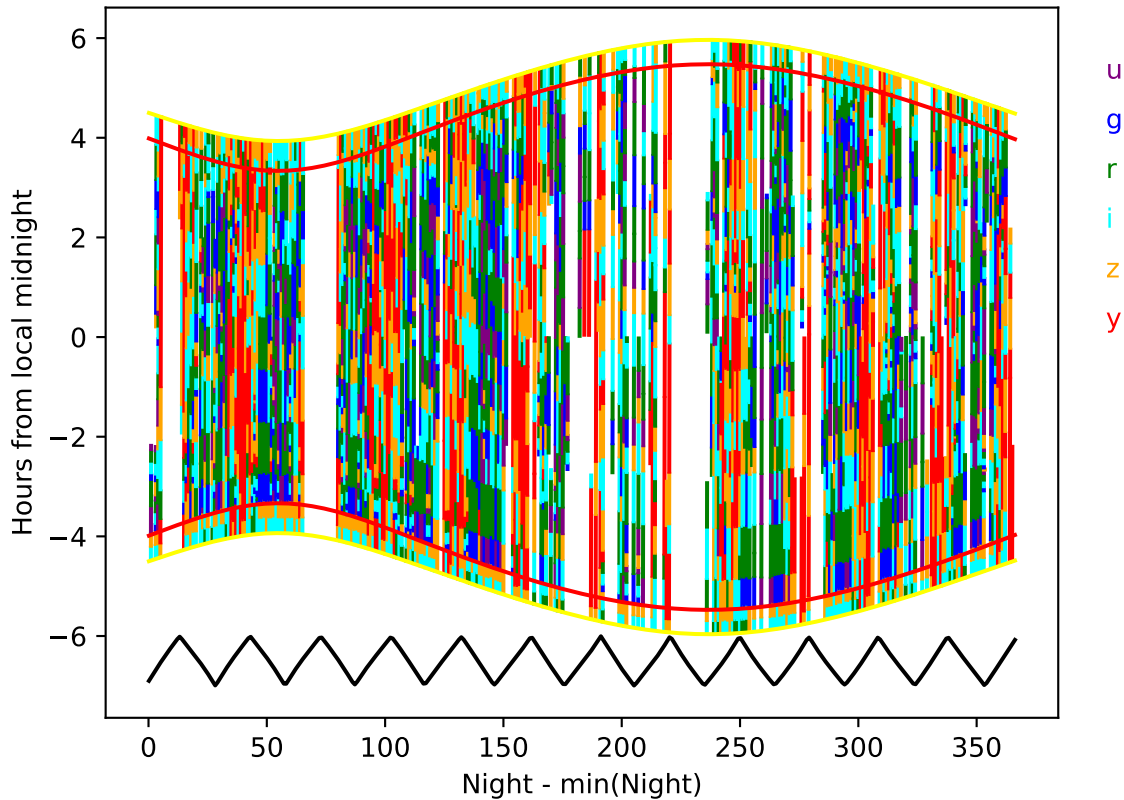
start_date_do180v3.4_10yrs year 5-6: Hourglass
