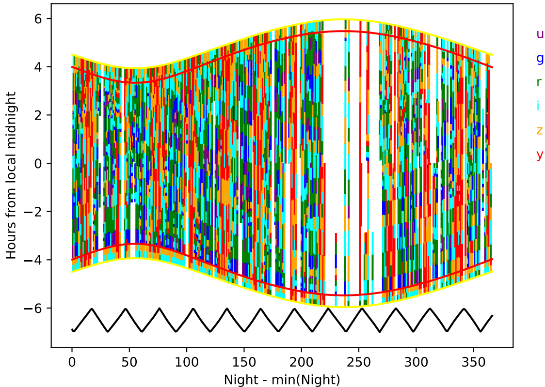
start_date_do180v3.4_10yrs year 2-3: Hourglass
