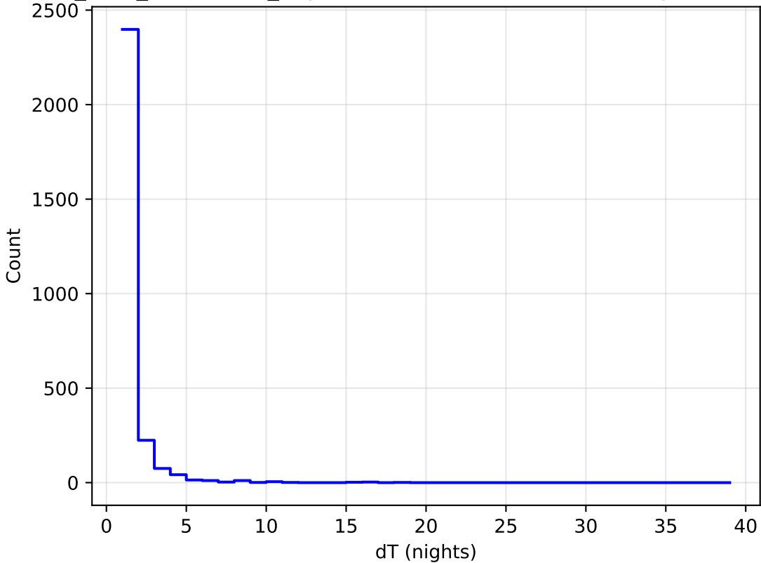
start_date_do180v3.4_10yrs all bands: DD:WFD Delta Nights Histogram
