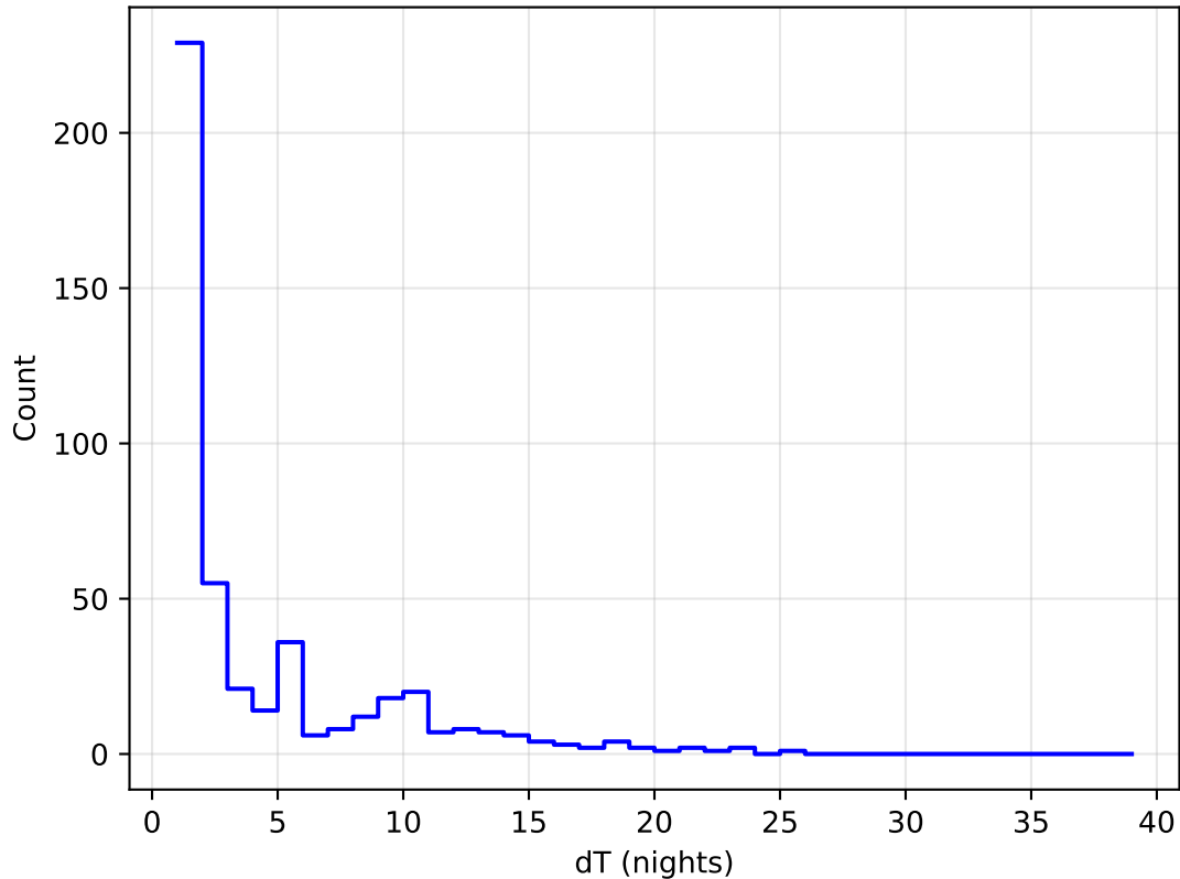
start_date_do180v3.4_10yrs all bands: DD: COSMOS Delta Nights Histogram
