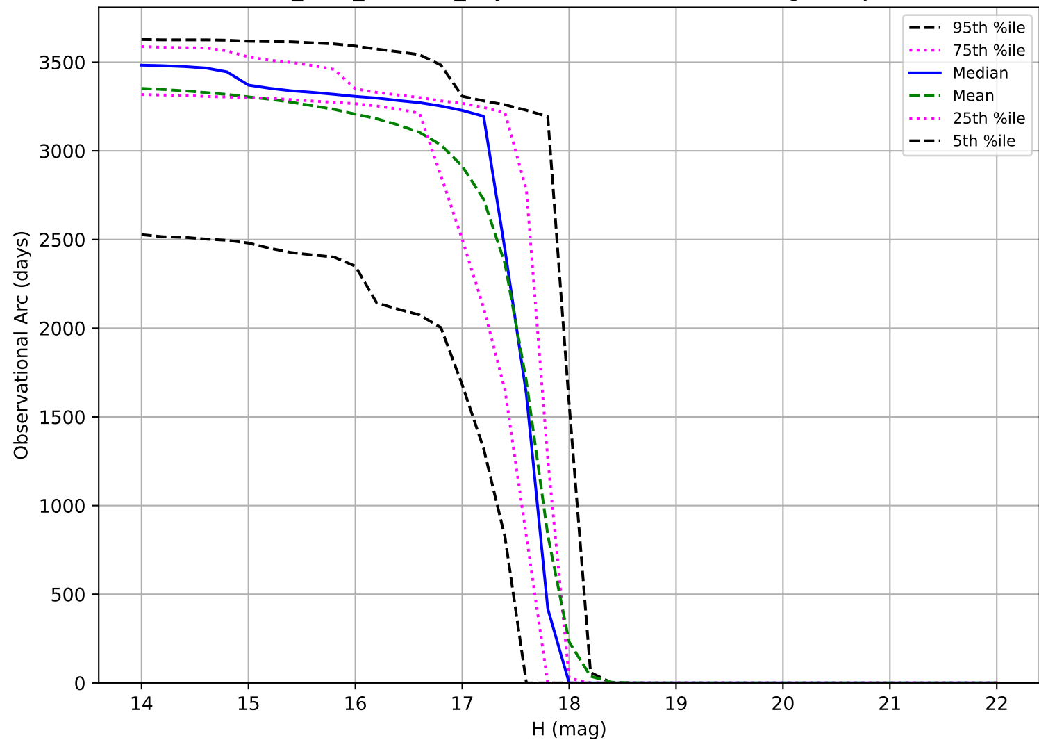
start_date_do0v3.4_10yrs: Observational Arc Length Trojan
