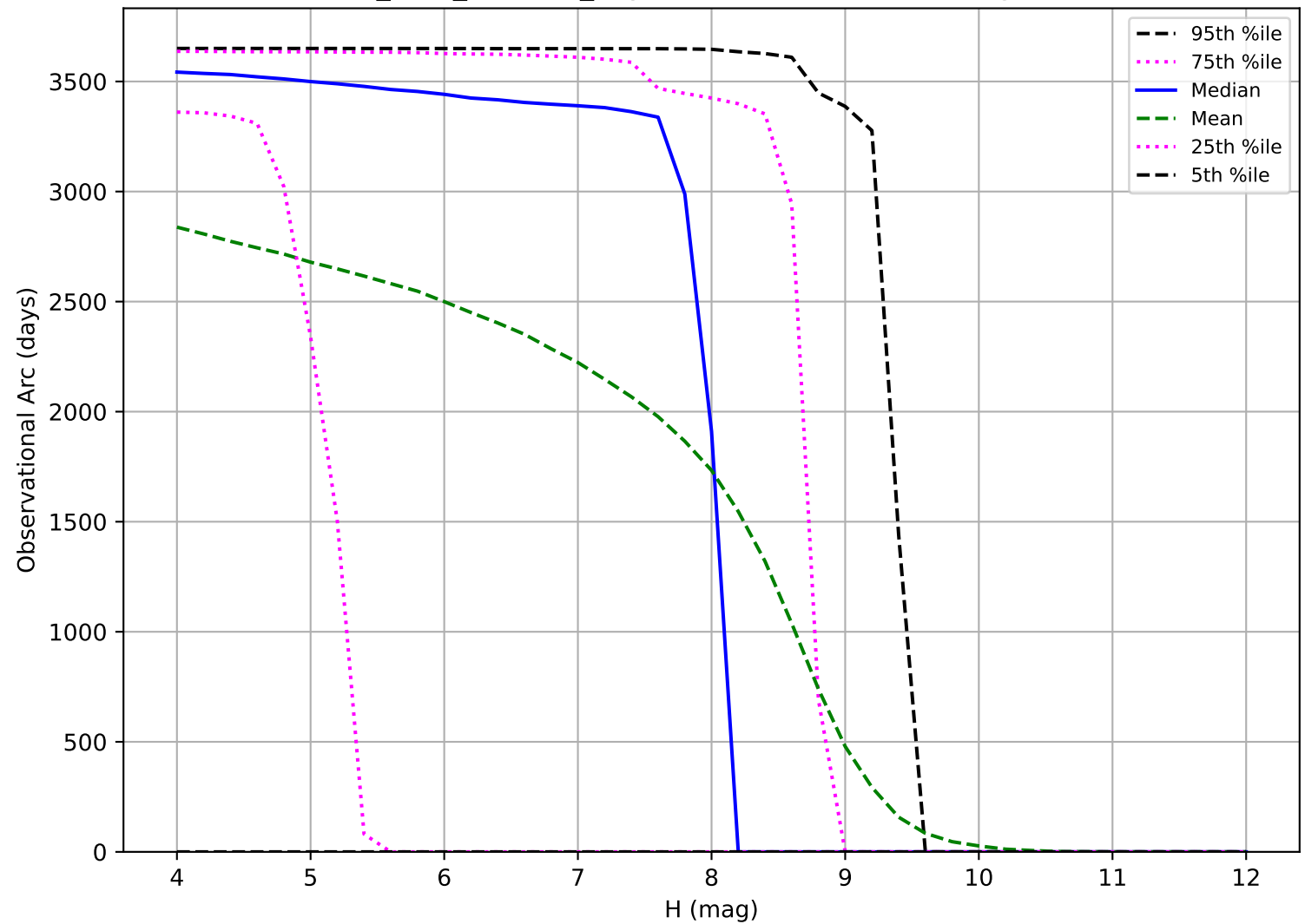
start_date_do0v3.4_10yrs: Observational Arc Length TNO
