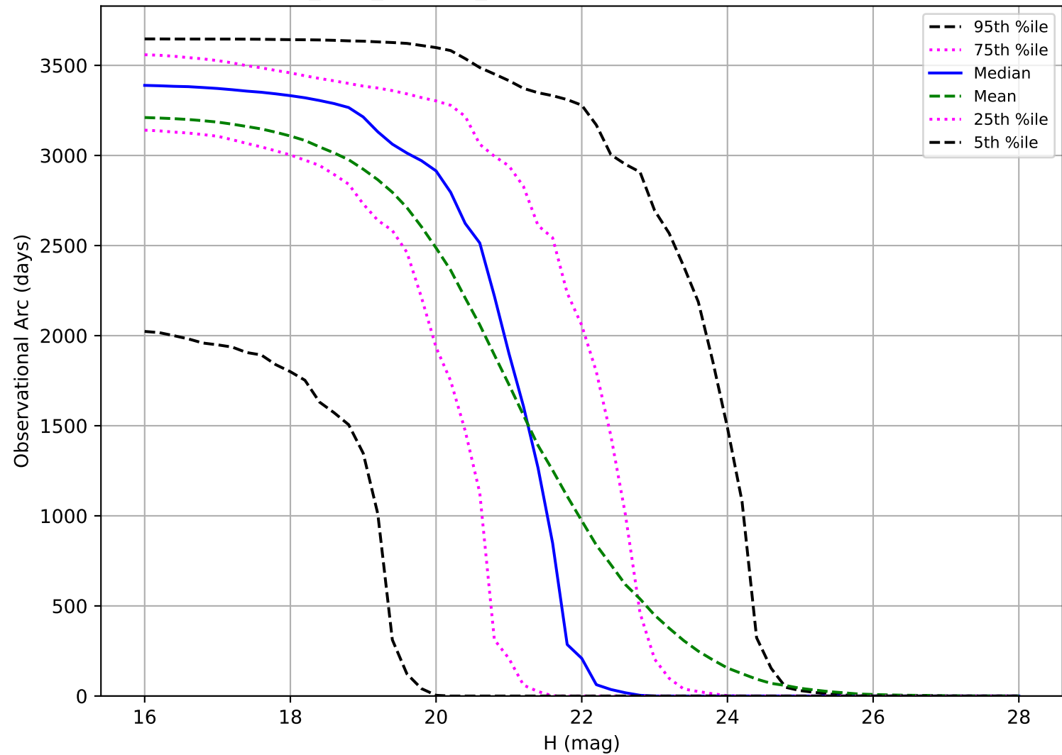
start_date_do0v3.4_10yrs: Observational Arc Length PHA
