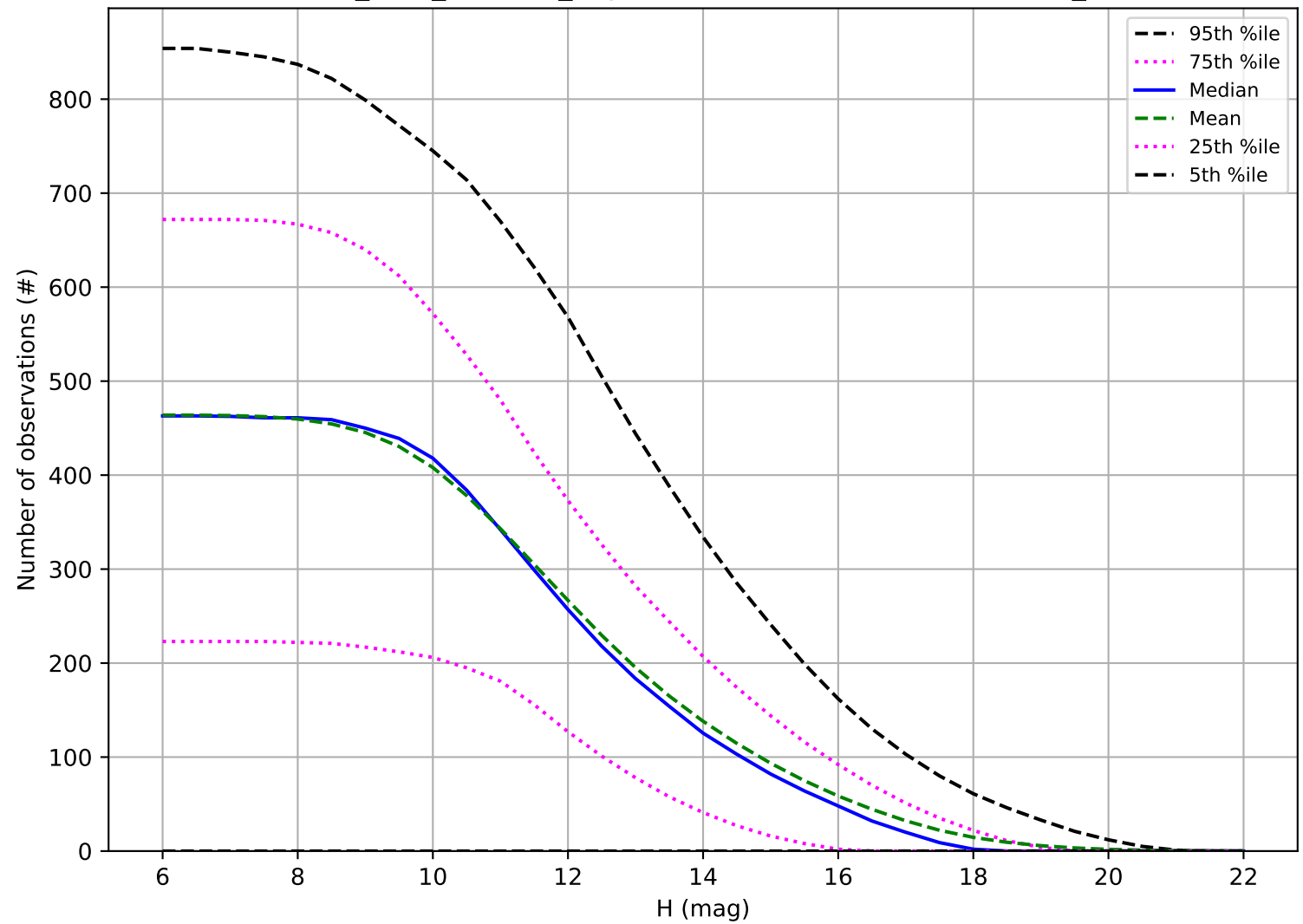
start_date_do0v3.4_10yrs: Number of observations OCC_r5
