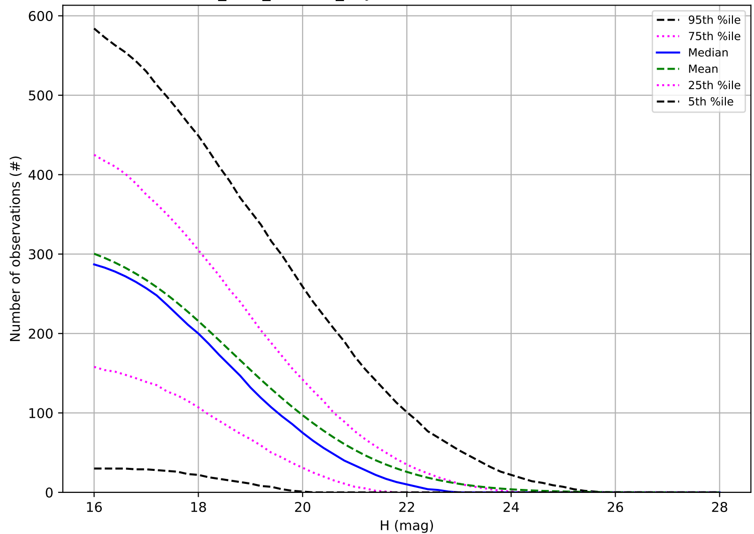
start_date_do0v3.4_10yrs: Number of observations NEO
