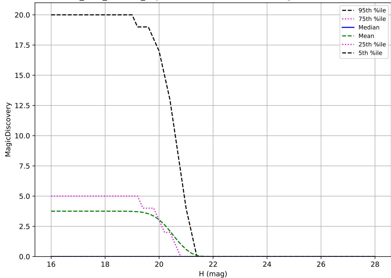
start_date_do0v3.4_10yrs: Vatira 6 detections in 60 nights detection loss
