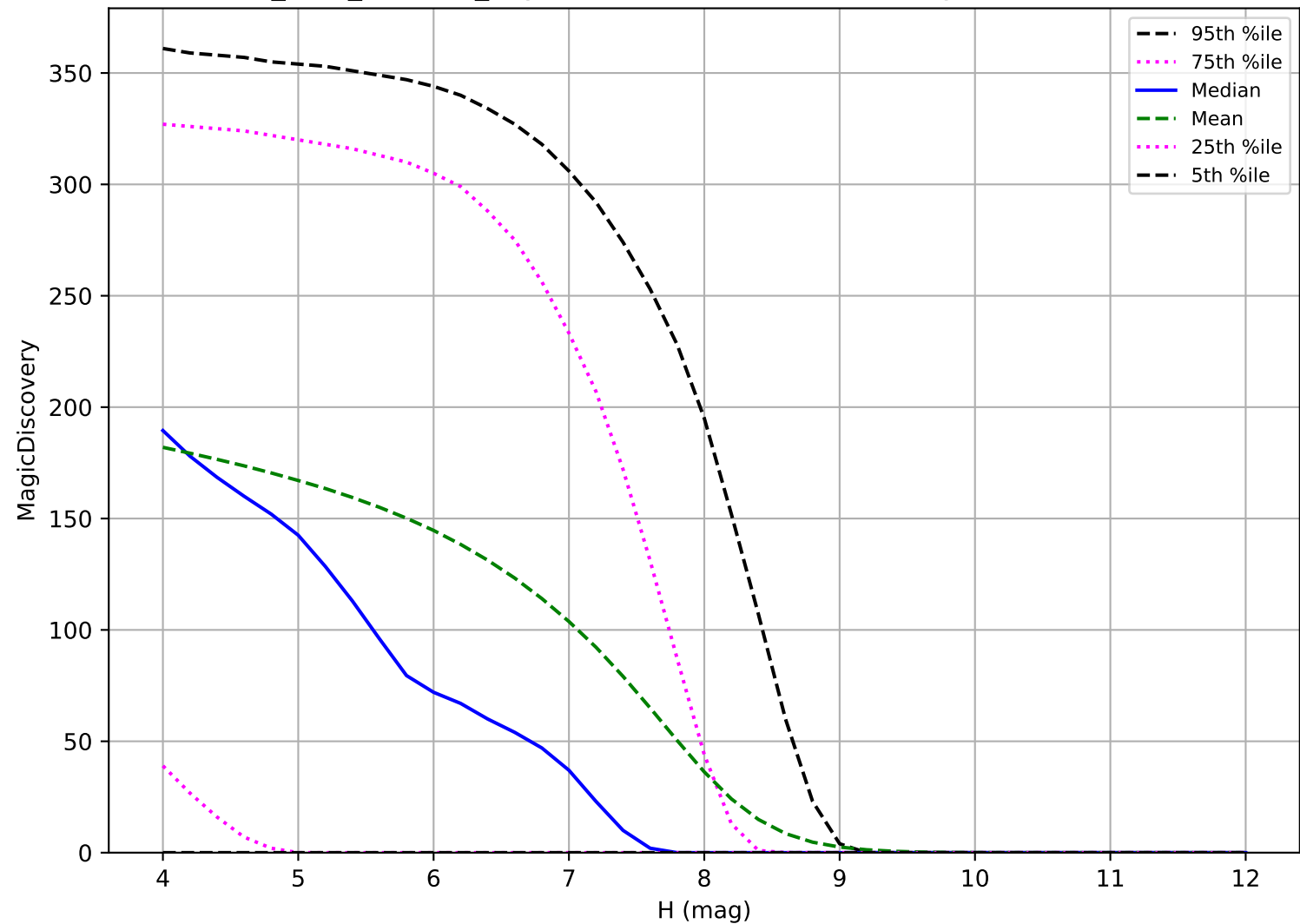
start_date_do0v3.4_10yrs: TNO 6 detections in 60 nights detection loss
