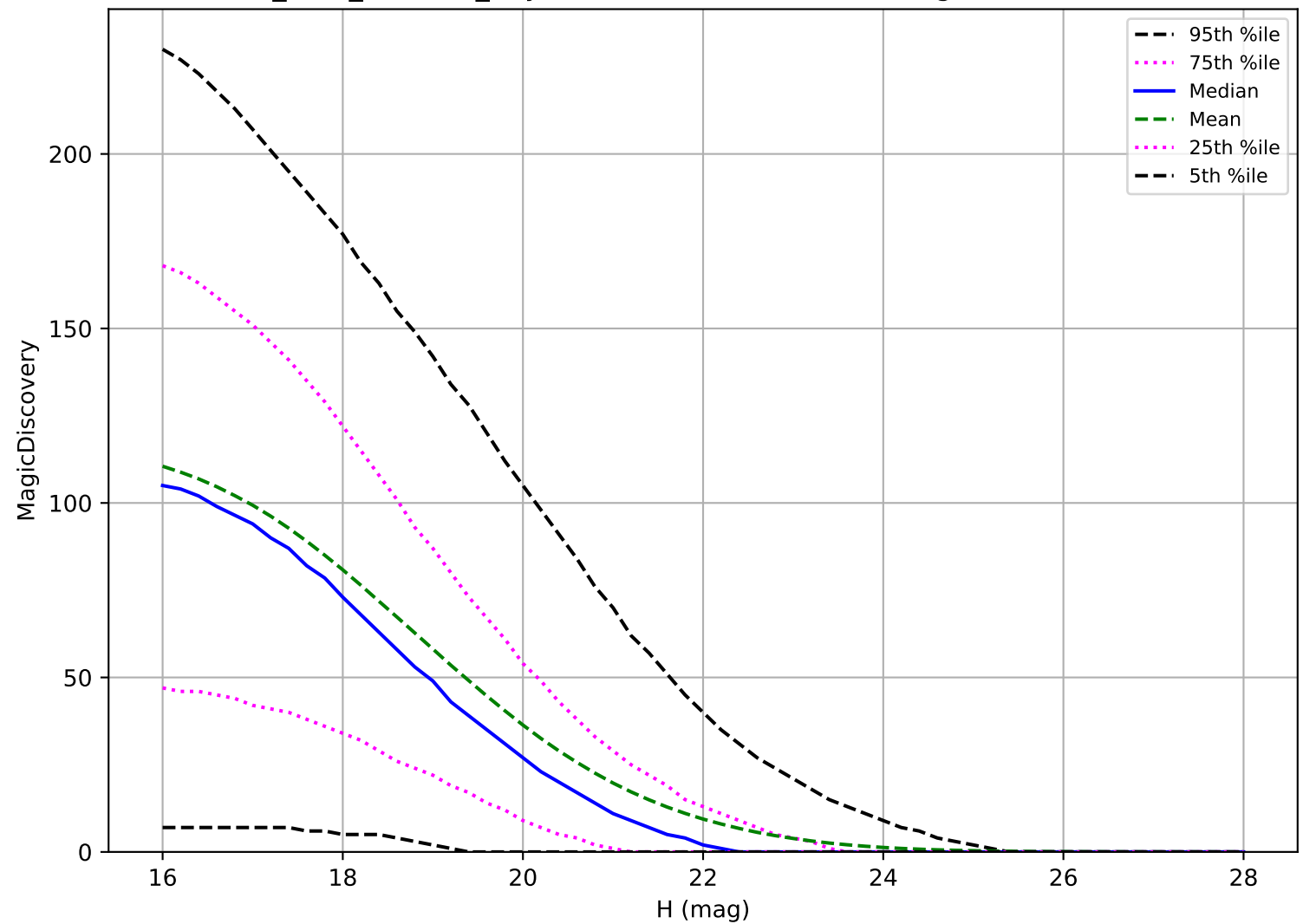
start_date_do0v3.4_10yrs: PHA 6 detections in 60 nights detection loss
