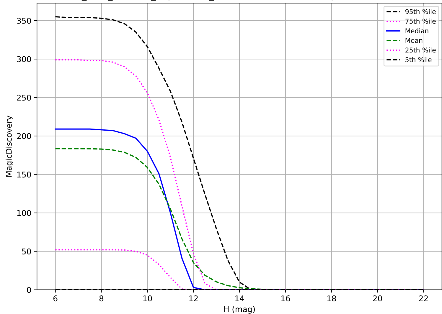
start_date_do0v3.4_10yrs: OCC_r20 6 detections in 60 nights detection loss
