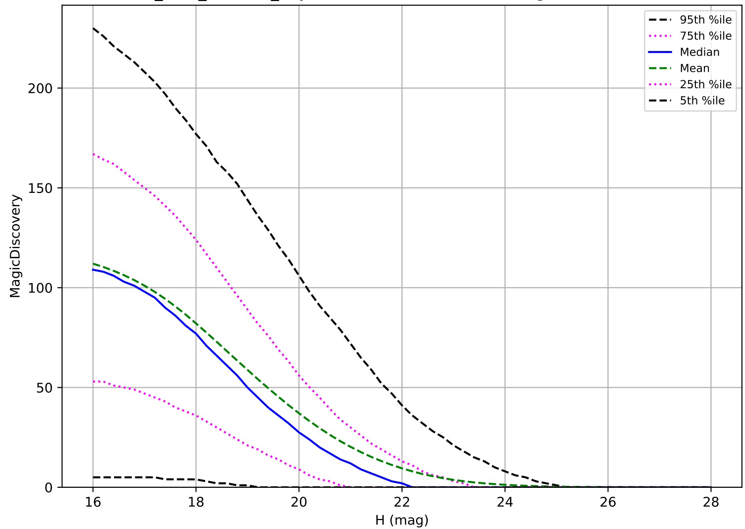
start_date_do0v3.4_10yrs: NEO 6 detections in 60 nights detection loss
