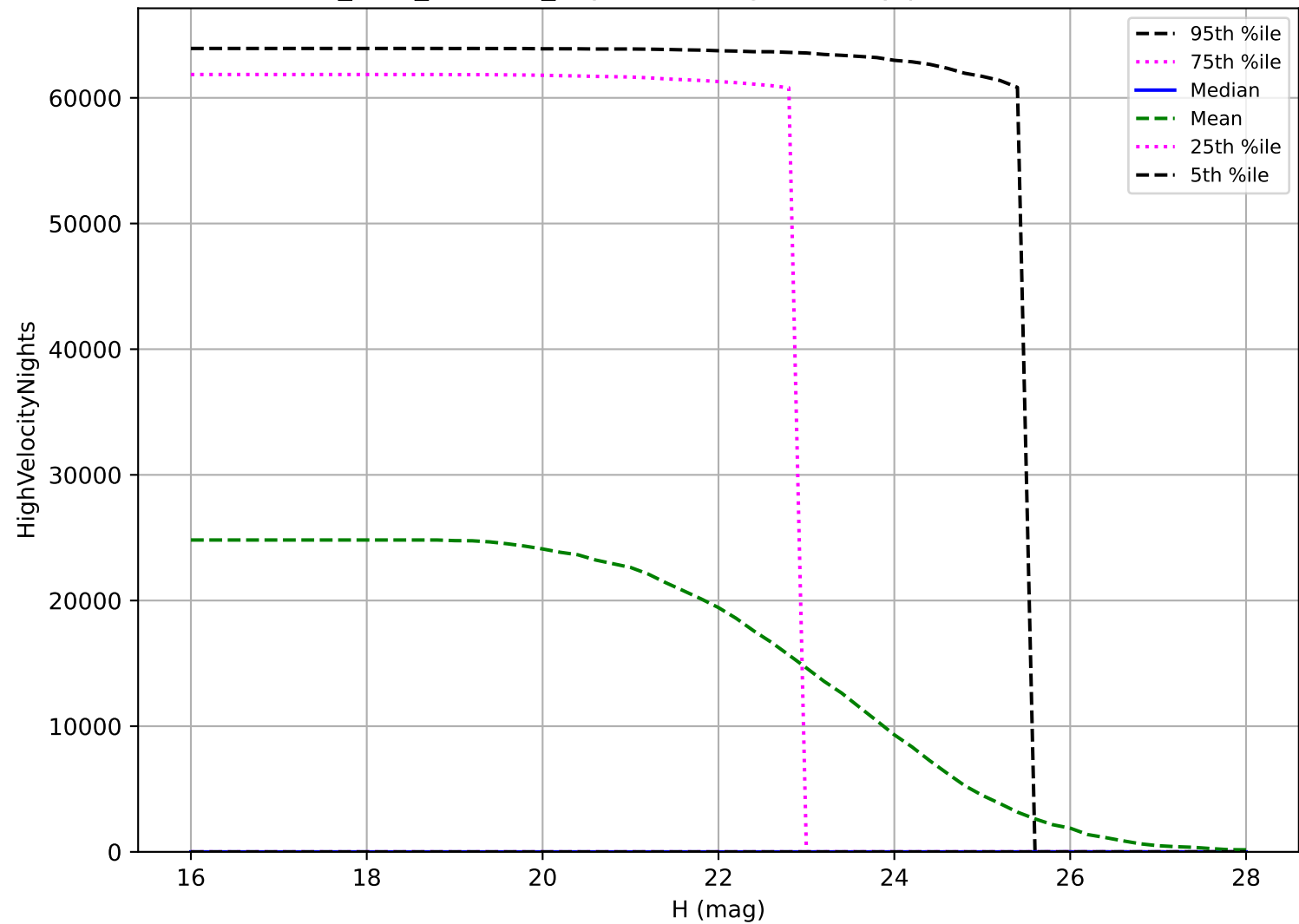
start_date_do0v3.4_10yrs: PHA High velocity pair detection loss
