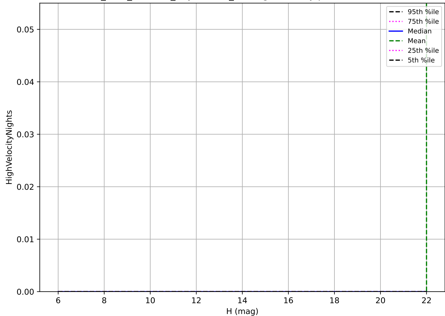
start_date_do0v3.4_10yrs: OCC_r20 High velocity pair detection loss
