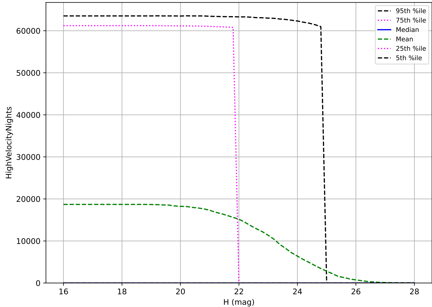
start_date_do0v3.4_10yrs: NEO High velocity pair detection loss
