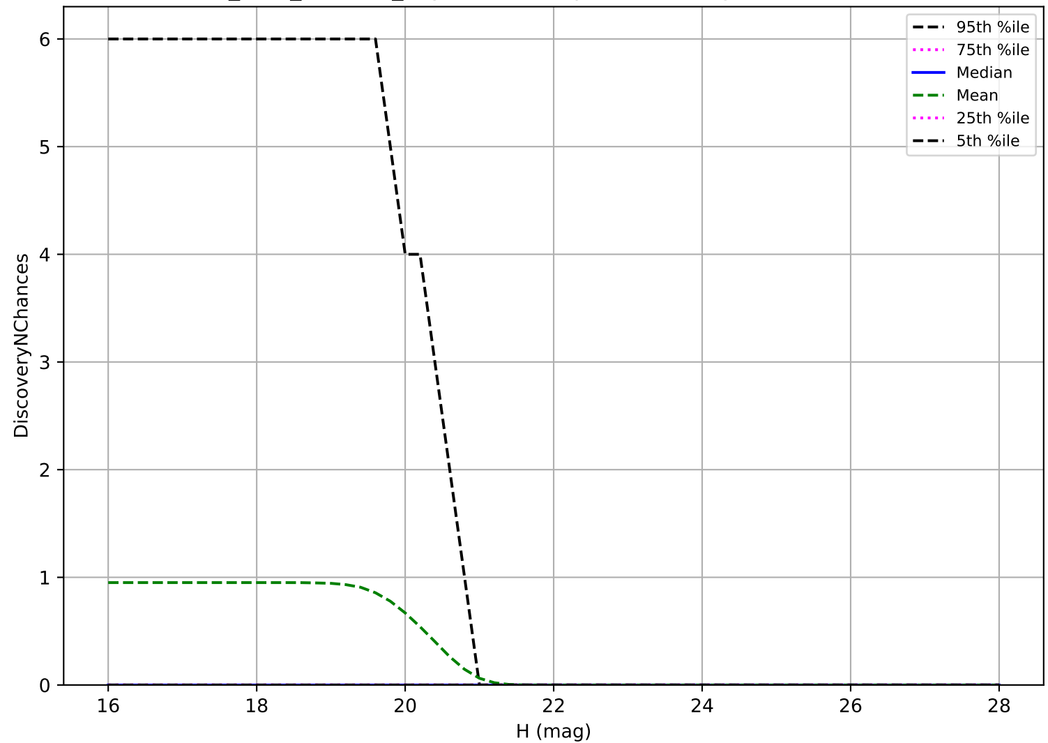
start_date_do0v3.4_10yrs: Vatira 3 pairs in 15 nights detection loss
