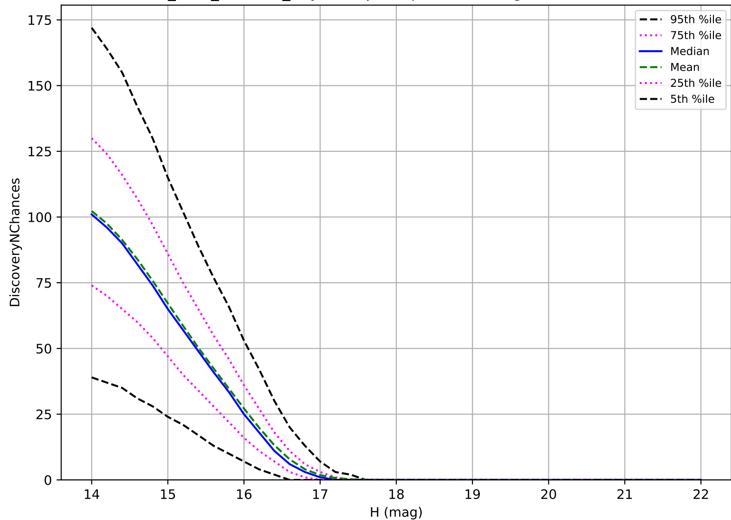
start_date_do0v3.4_10yrs: Trojan 3 pairs in 15 nights detection loss
