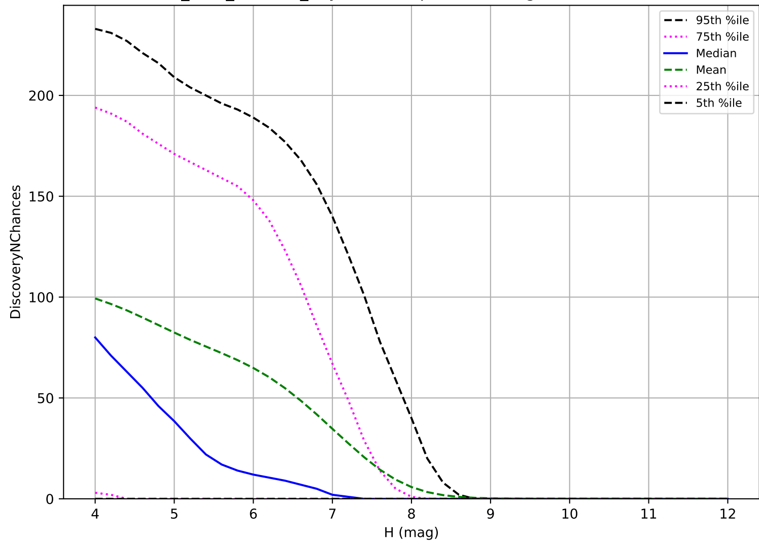
start_date_do0v3.4_10yrs: TNO 3 pairs in 15 nights detection loss
