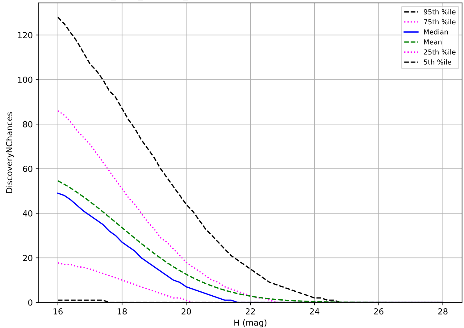
start_date_do0v3.4_10yrs: PHA 3 pairs in 15 nights detection loss
