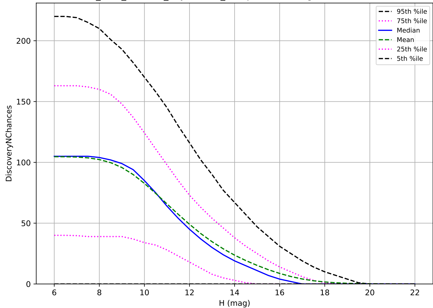
start_date_do0v3.4_10yrs: OCC_r5 3 pairs in 15 nights detection loss
