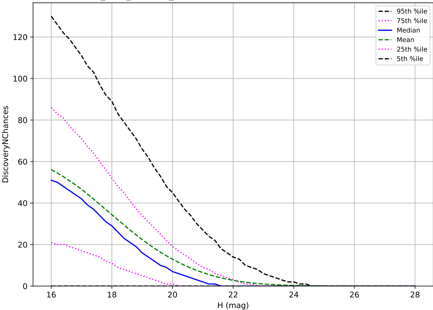
start_date_do0v3.4_10yrs: NEO 3 pairs in 15 nights detection loss
