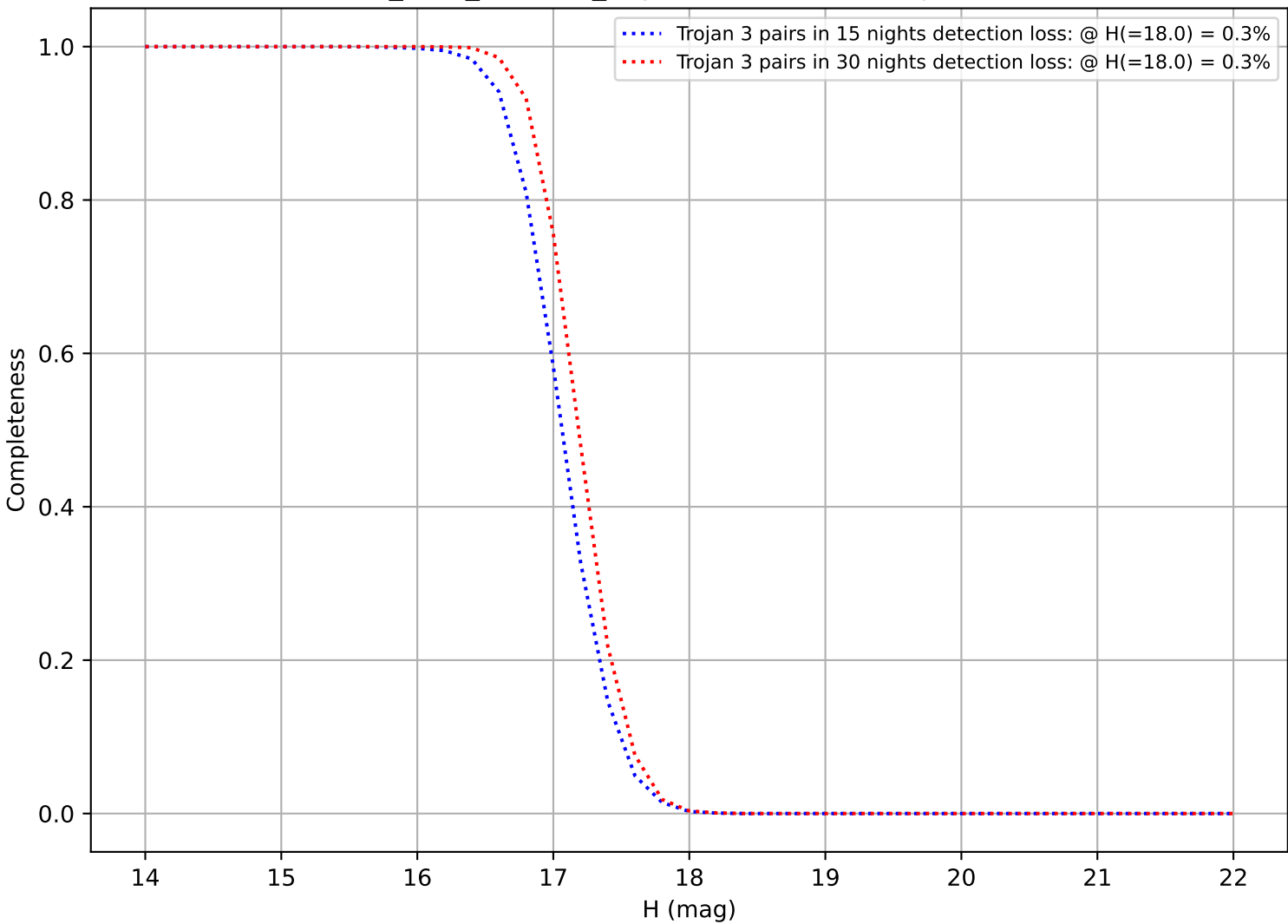
start_date_do0v3.4_10yrs: DifferentialCompleteness
