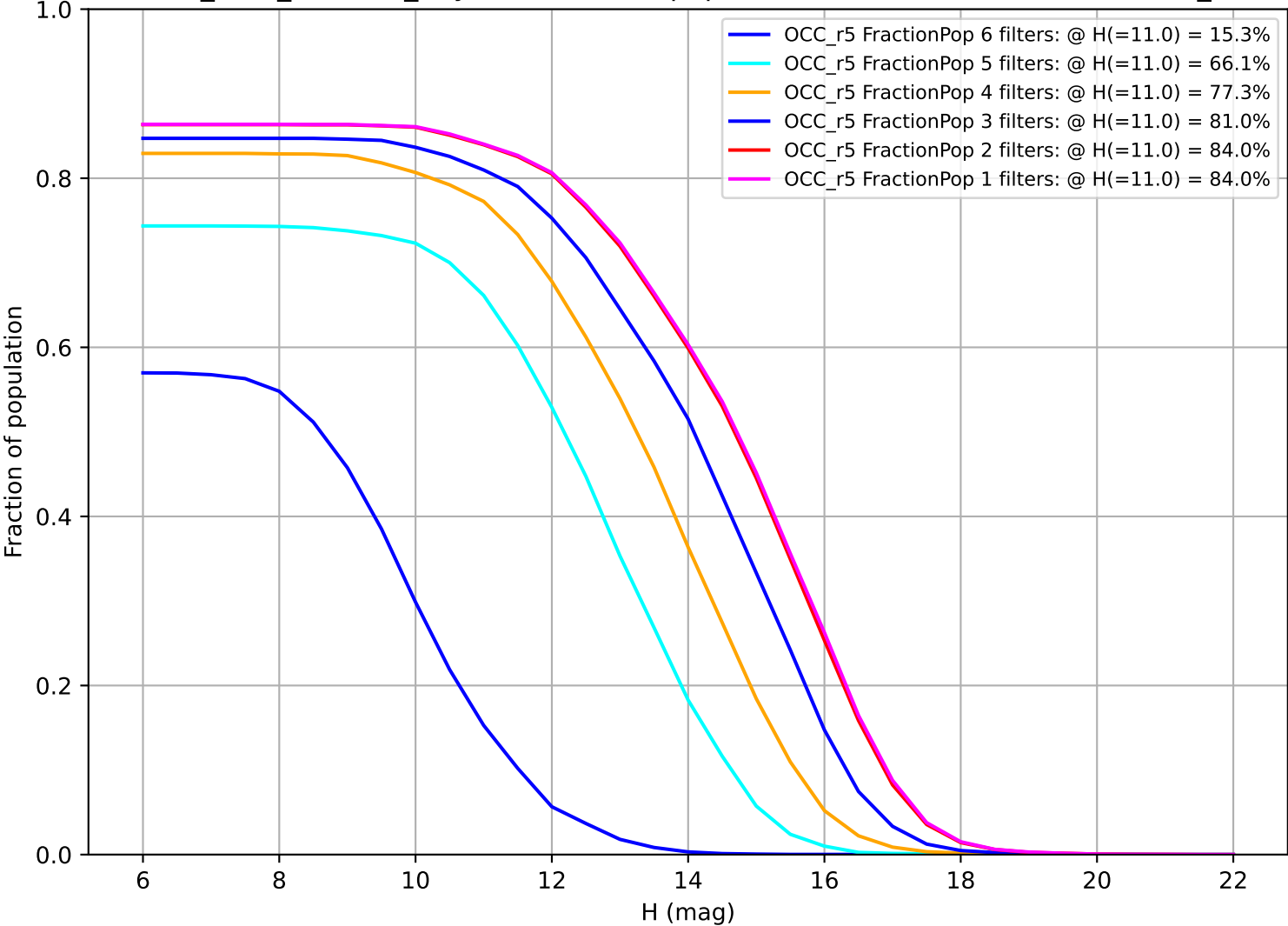
start_date_do0v3.4_10yrs: Fraction of population with colors in X filters OCC_r5
