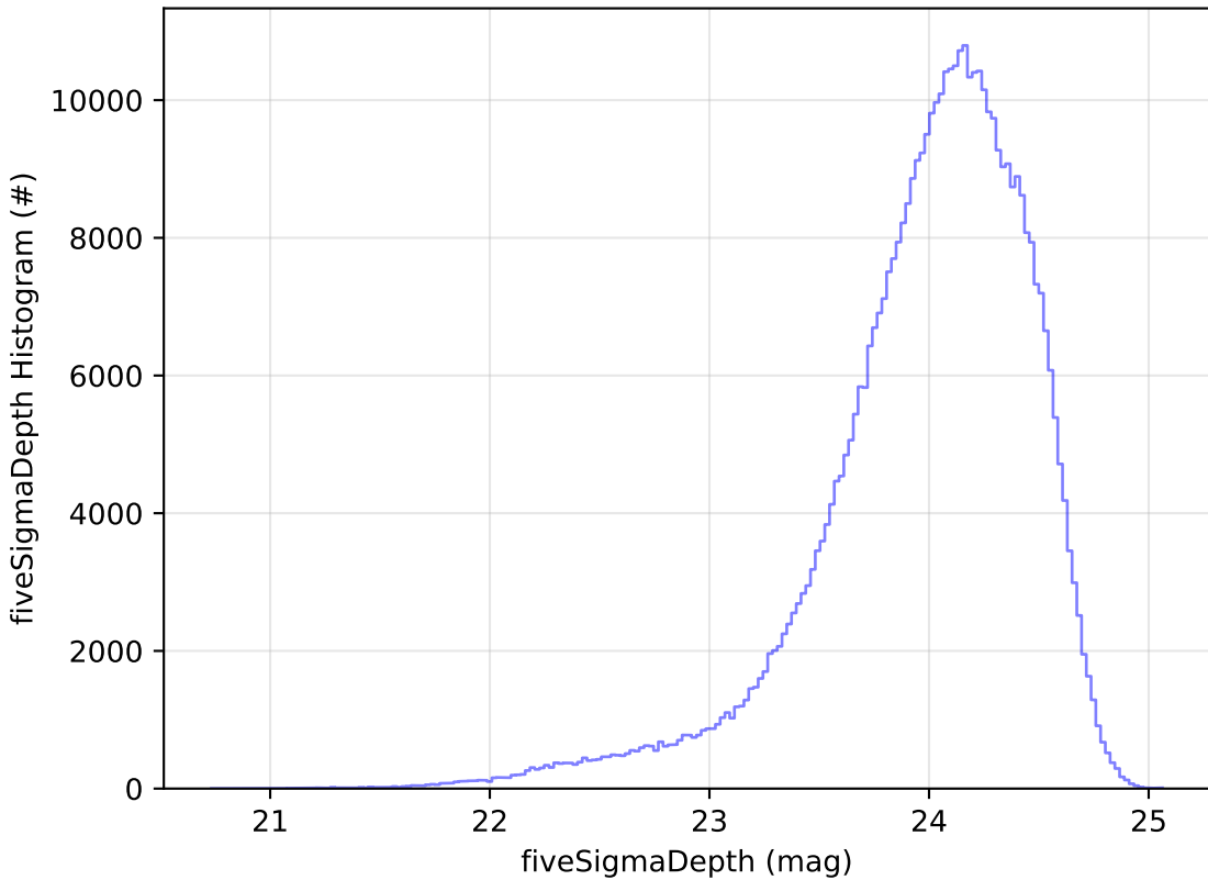
start_date_do0v3.4_10yrs r: fiveSigmaDepth Histogram
