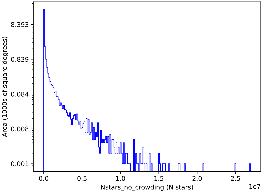
start_date_do0v3.4_10yrs i: Nstars_no_crowding
