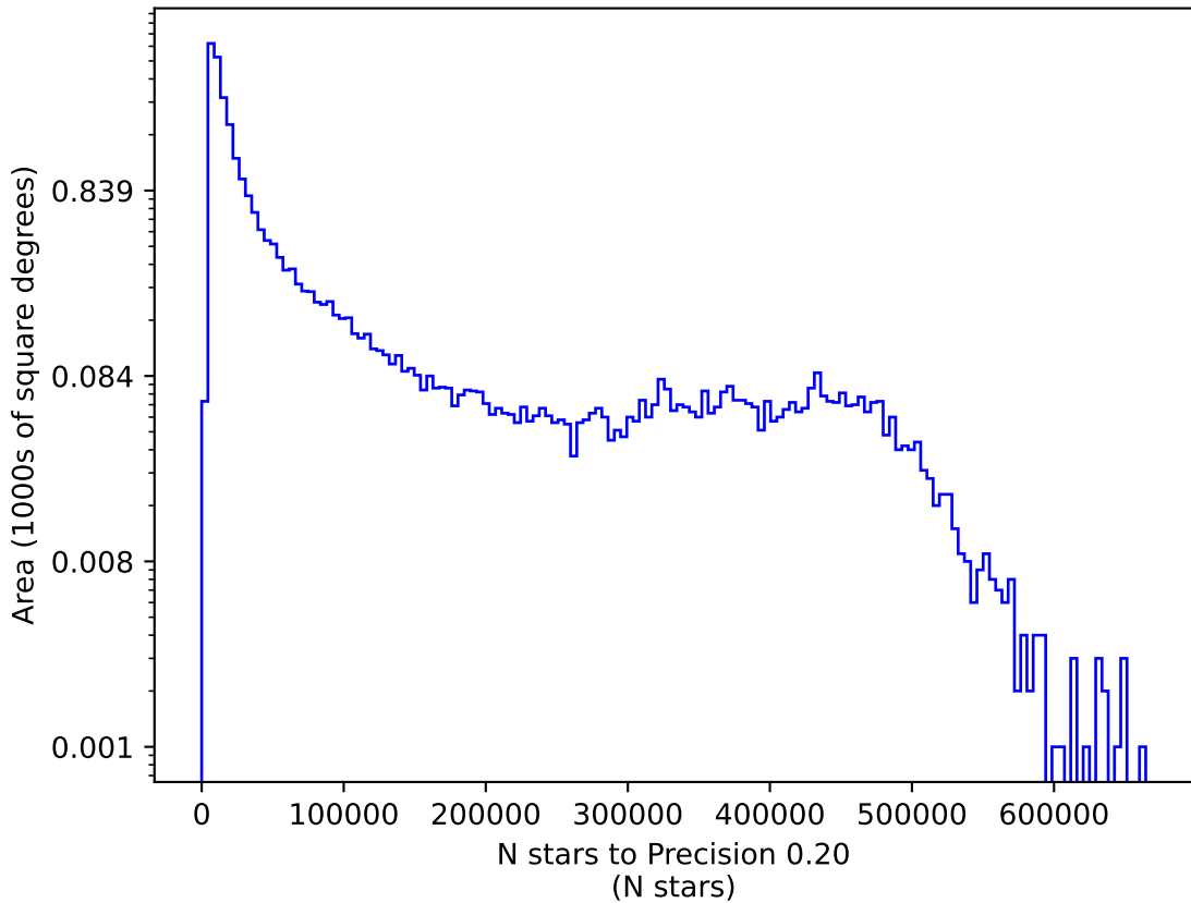
start_date_do0v3.4_10yrs r: N stars to Precision 0.20
