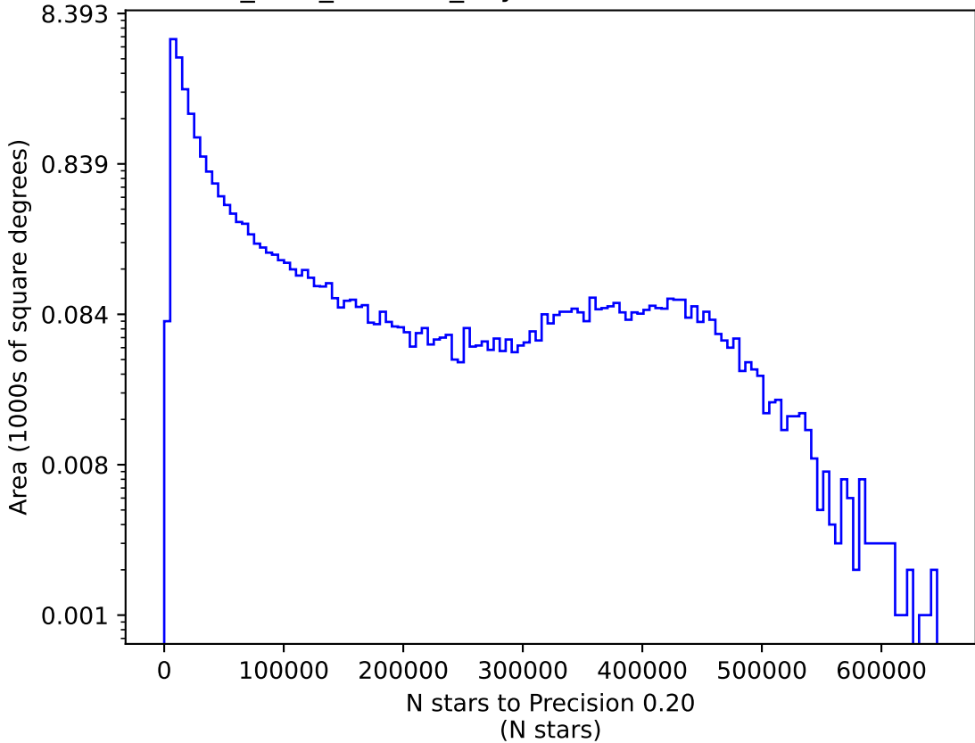
start_date_do0v3.4_10yrs i: N stars to Precision 0.20
