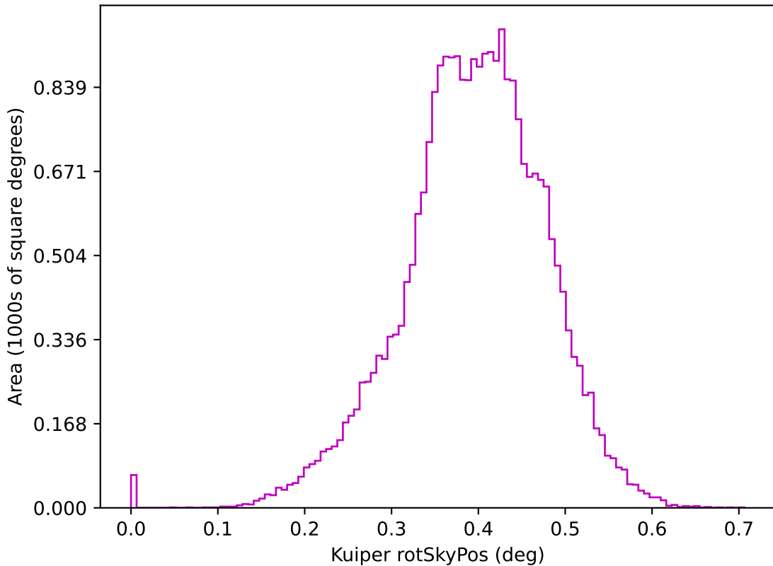
start_date_do0v3.4_10yrs z: Kuiper rotSkyPos
