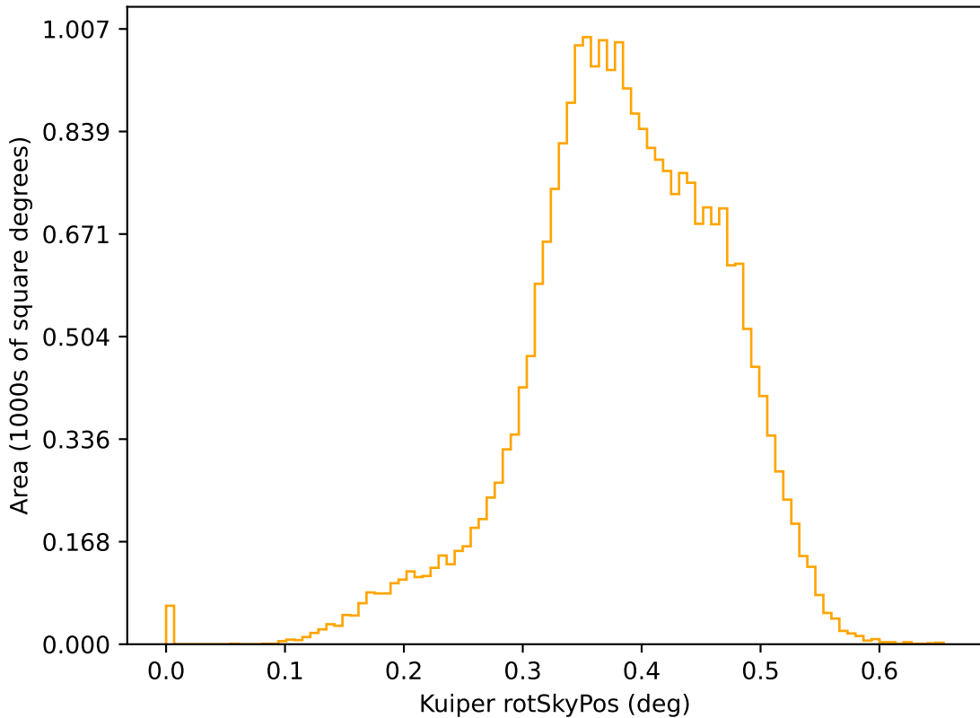
start_date_do0v3.4_10yrs r: Kuiper rotSkyPos
