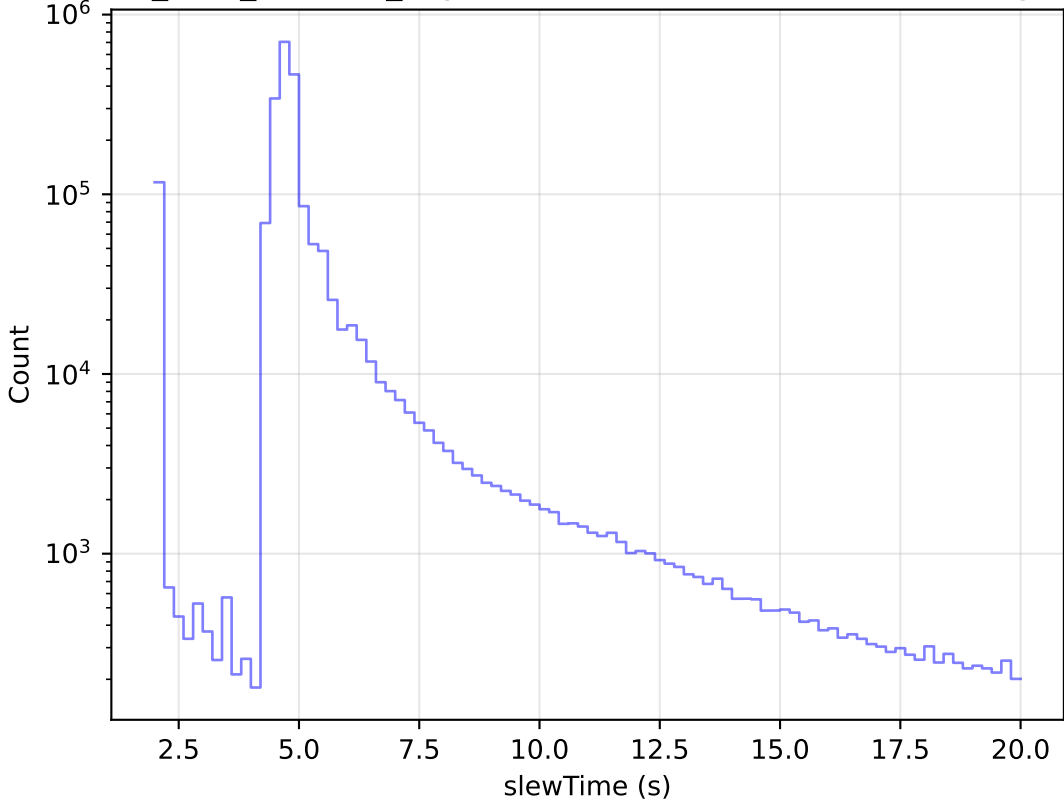
start_date_do0v3.4_10yrs All visits: Zoom Slew Time Histogram
