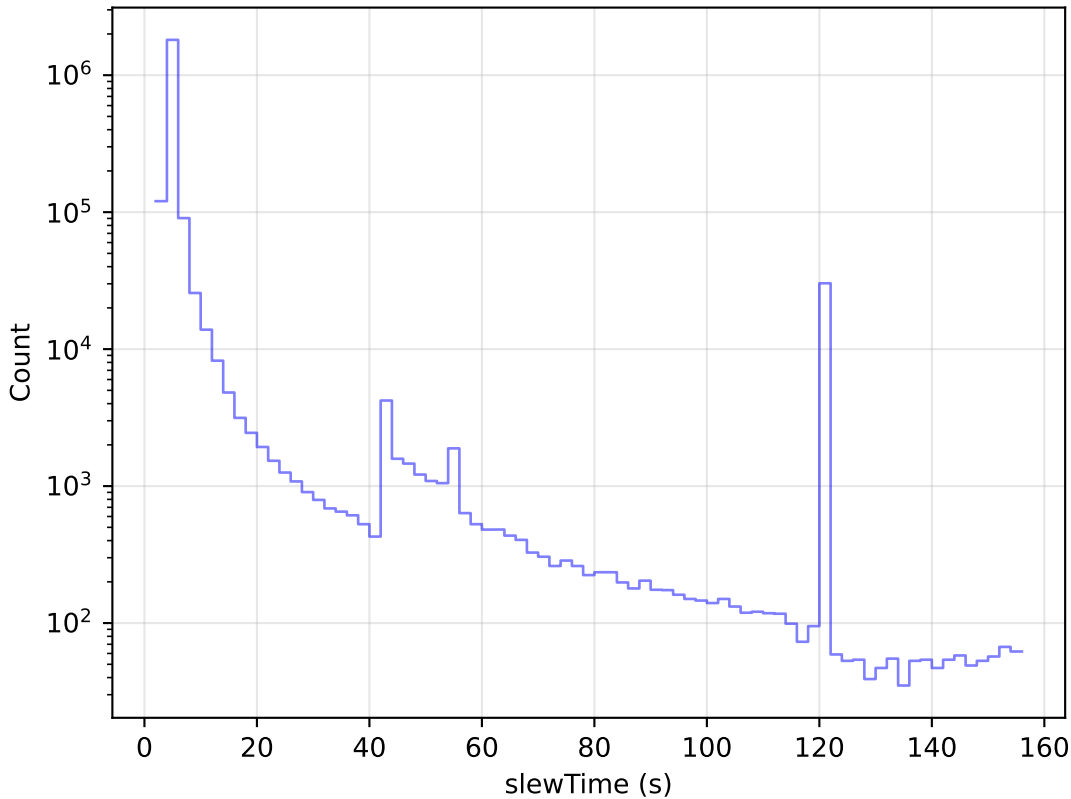
start_date_do0v3.4_10yrs All visits: Slew Time Histogram
