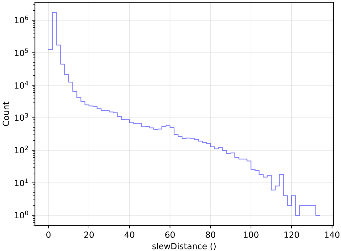
start_date_do0v3.4_10yrs All visits: Slew Distance Histogram
