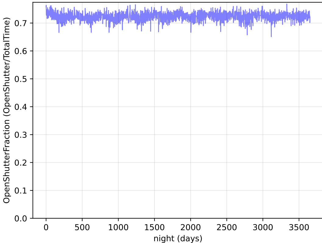
start_date_do0v3.4_10yrs : OpenShutterFraction
