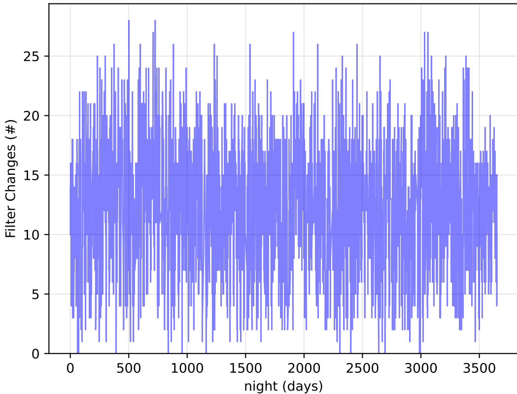
start_date_do0v3.4_10yrs : Filter Changes
