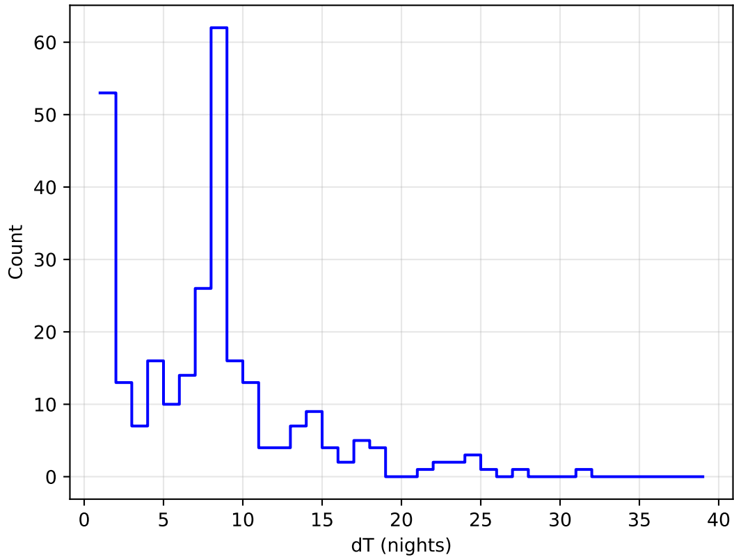
start_date_do0v3.4_10yrs all bands: DD:XMM_LSS Delta Nights Histogram
