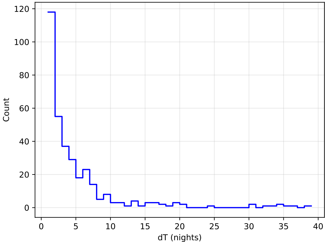
start_date_do0v3.4_10yrs all bands: DD:WFD Delta Nights Histogram
