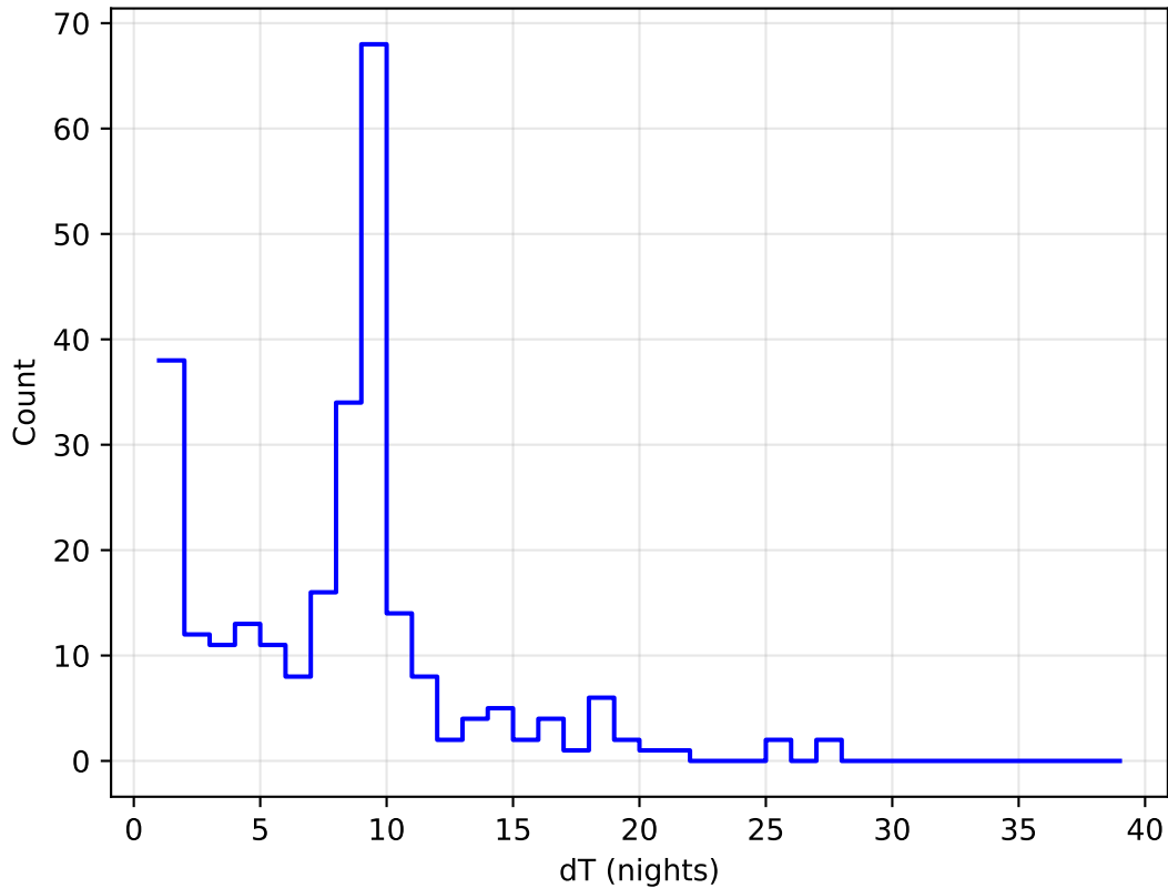
start_date_do0v3.4_10yrs all bands: DD:ELAISS1 Delta Nights Histogram
