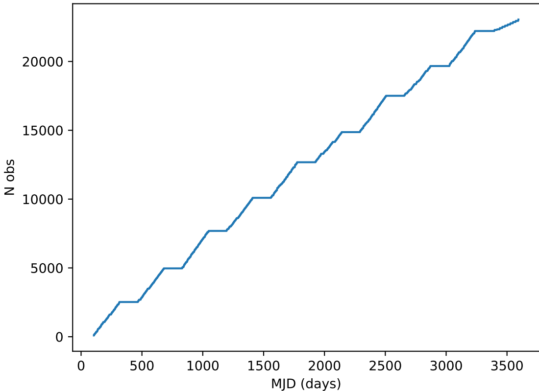
start_date_do0v3.4_10yrs all bands: DD:EDFS Cumulative NVisits
