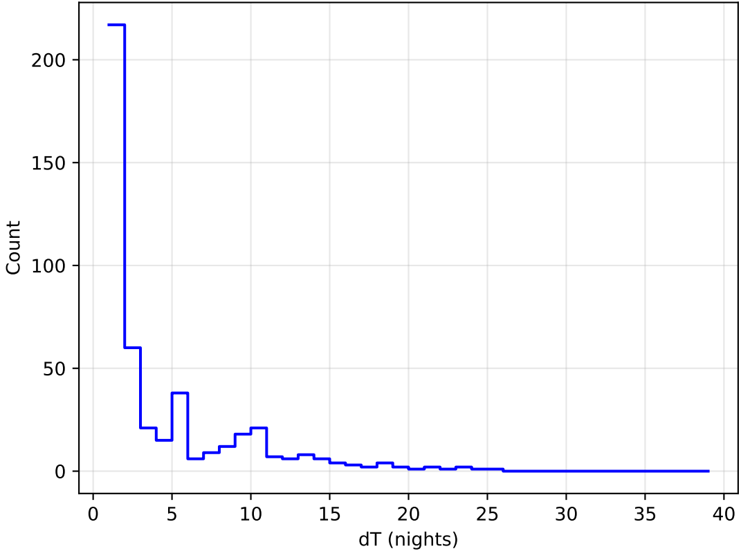
start_date_do0v3.4_10yrs all bands: DD: COSMOS Delta Nights Histogram
