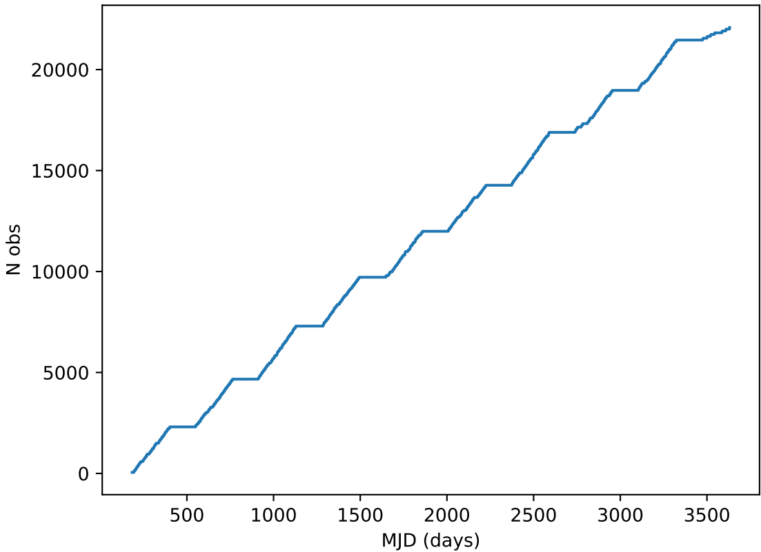
start_date_do-90v3.4_10yrs all bands: DD:ECDFS Cumulative NVisits
